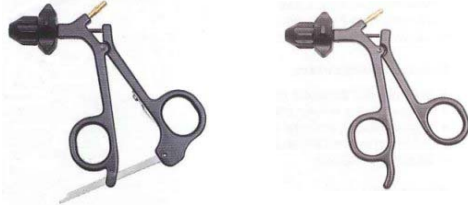
Standard handle ref: 48200185 Ratchet Handle ref: 48200187 Rotatable outer sheath 5mm 35cm ref: 48200002SA
